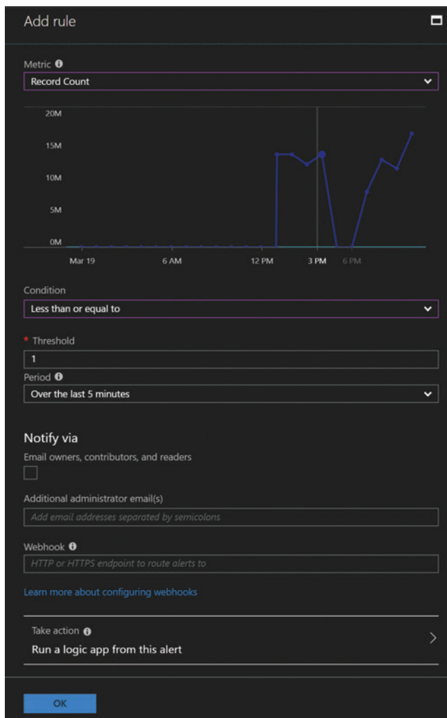
Figure 9 Setting Up an Alert on Metric
