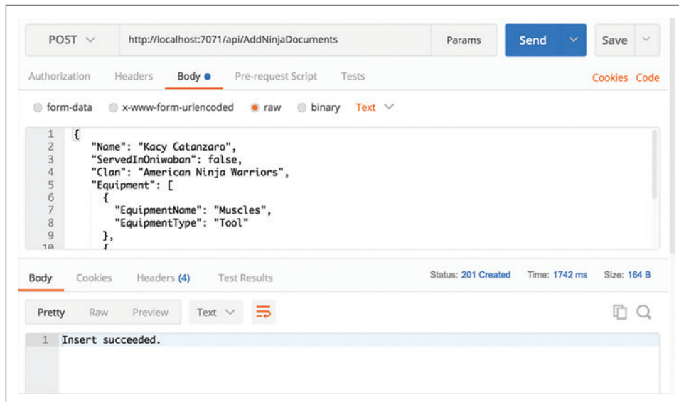
Figure 5 Creating a Request to Call the AddNinjaDocuments Function
