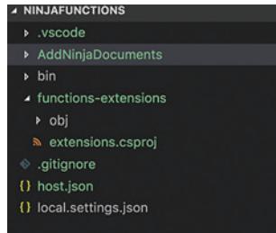
Figure 2 The New Functions-Extensions Folder to House the Cosmos DB Extension
