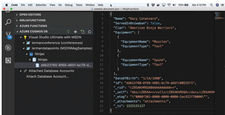
Figure 6 The New Document as Displayed by the Cosmos DB Extension
